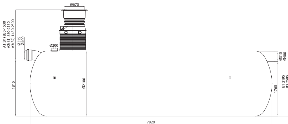
SANDTRAP G 20000/315, 20000/400
