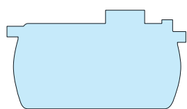
MIRI OAS-1
