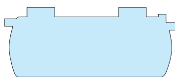
MIRI OAS-2
