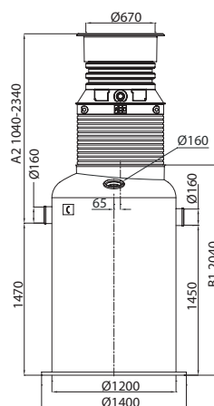
OLEOPATOR G 6/1200
